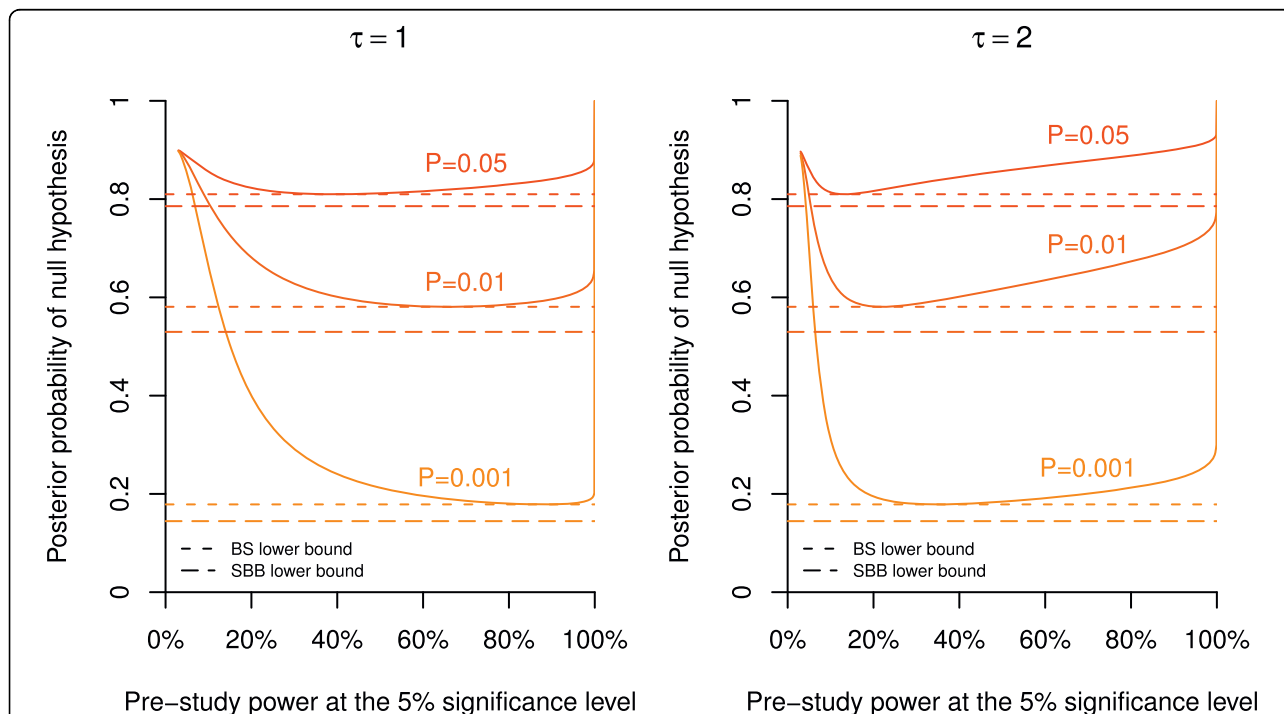
Figure 4 Dependence of the posterior probability on study power. Posterior probability of the null hypothesis plotted against the (pre-study) power at the 5% significance level for P = 0.05, 0.01, and 0.001 and a prior probability of q = 90\% . The calculation is based on a normal prior with standard deviation \tau = 1 (left plot) and \tau = 2 (right plot) under the alternative, assuming that one unit corresponds to the minimum clinically important difference. The dashed lines indicate the minimum posterior probability as obtained from the BS (short dashed) and SBB (long dashed) approach, respectively.
