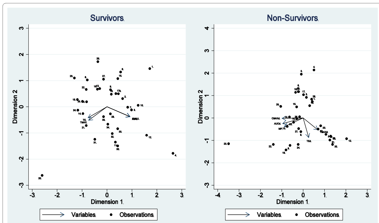
Figure 4 Biplots for survivors and non-survivors demonstrating the multivariate relationships between global performance indices. CMAX: peak hazard; TMAX: time to peak hazard; AUC: area under the hazard curve; KE: "elimination rate", TE: technical efficiency; MP: median mortality probability.
